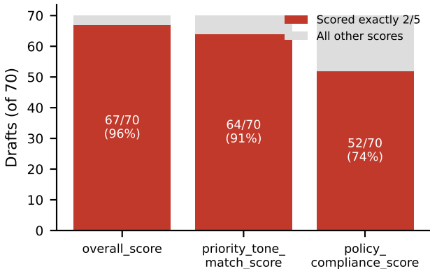
Judge scores clustering at 2/5 (prompt/rubric mismatch, see Sec. VI-D)
